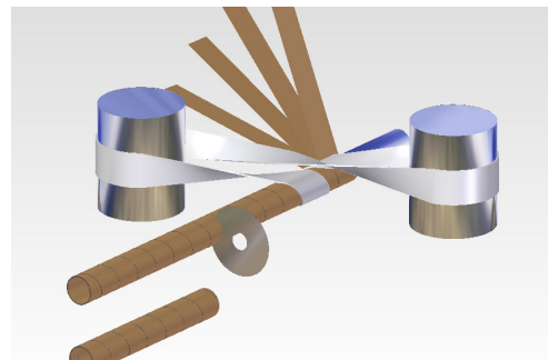
Diagram of the tube winding process
